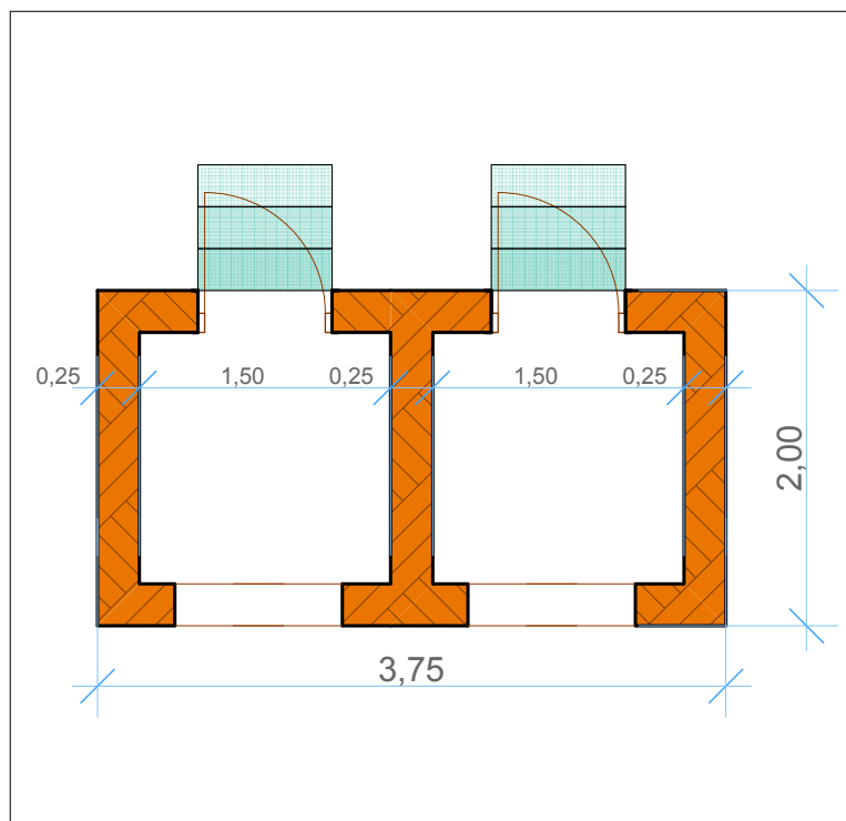
Plan Latrine Double
